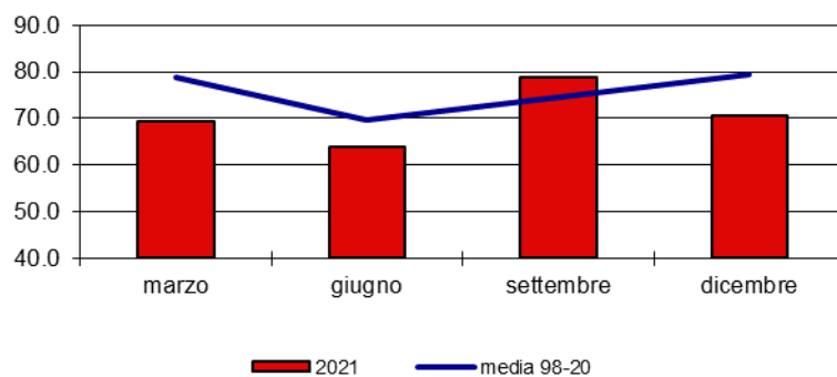
Clorofilla a (µg/l)
