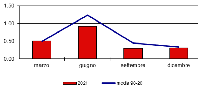
Clorofilla a (µg/l)
