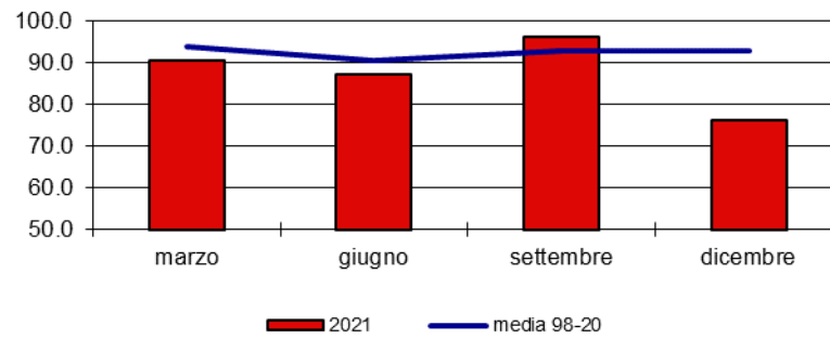
Clorofilla a (µg/l)
